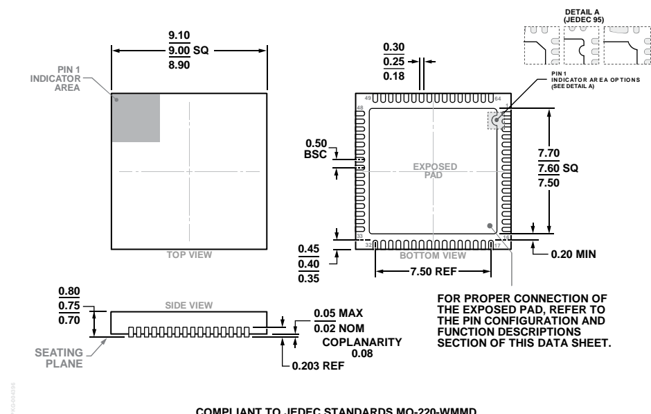
Figure 54. 64-Lead Lead Frame Chip Scale Package [LFCSP] 9 mm × 9 mm Body and 0.75 mm Package Height (CP-64-15) Dimensions shown in millimeters
