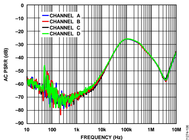
Figure 11. AC PSRR vs. Frequency
