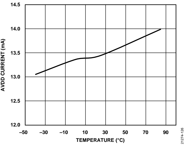
Figure 33. AVDD Current vs. Temperature
