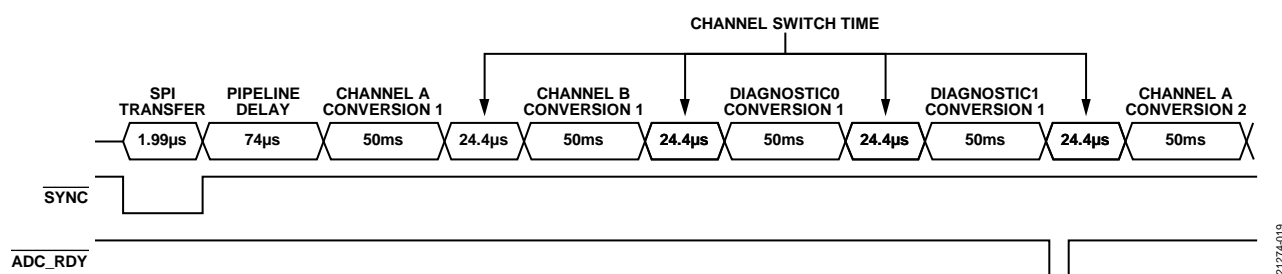
Figure 48. Multichannel, Continuous Conversions Timing Diagram
