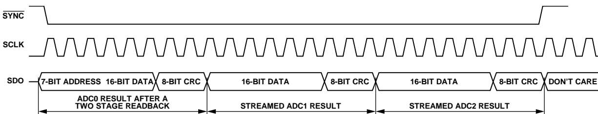
Figure 53. Streaming Mode SDO Contents
