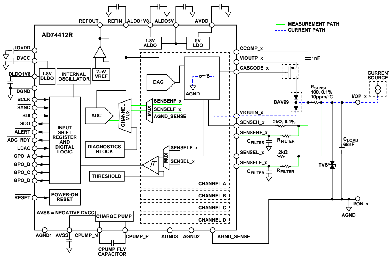
Figure 38. Current Input, Externally Powered Mode Configuration
