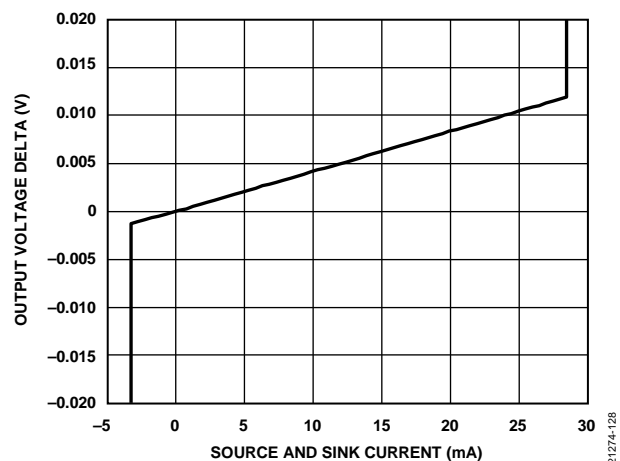
Figure 14. Output Voltage ( V_{\text{OUT}} ) Source and Sink Capability
