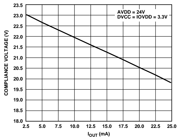
Figure 22. Compliance Voltage vs. I_{OUT}
